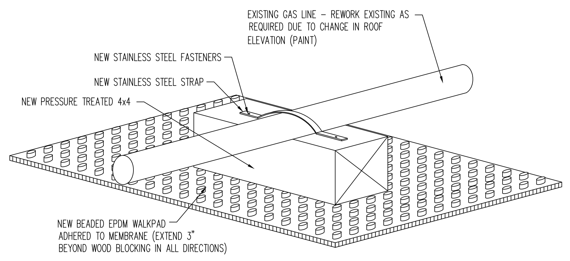
6 UTILITY LINE SUPPORT (AS REQUIRED) R2 | D4 NOT TO SCALE
