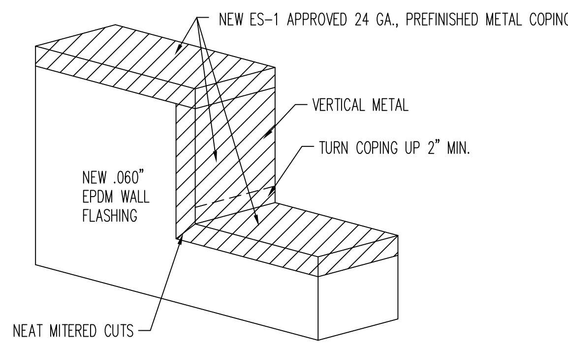
METAL COPING AT STEP DOWN
