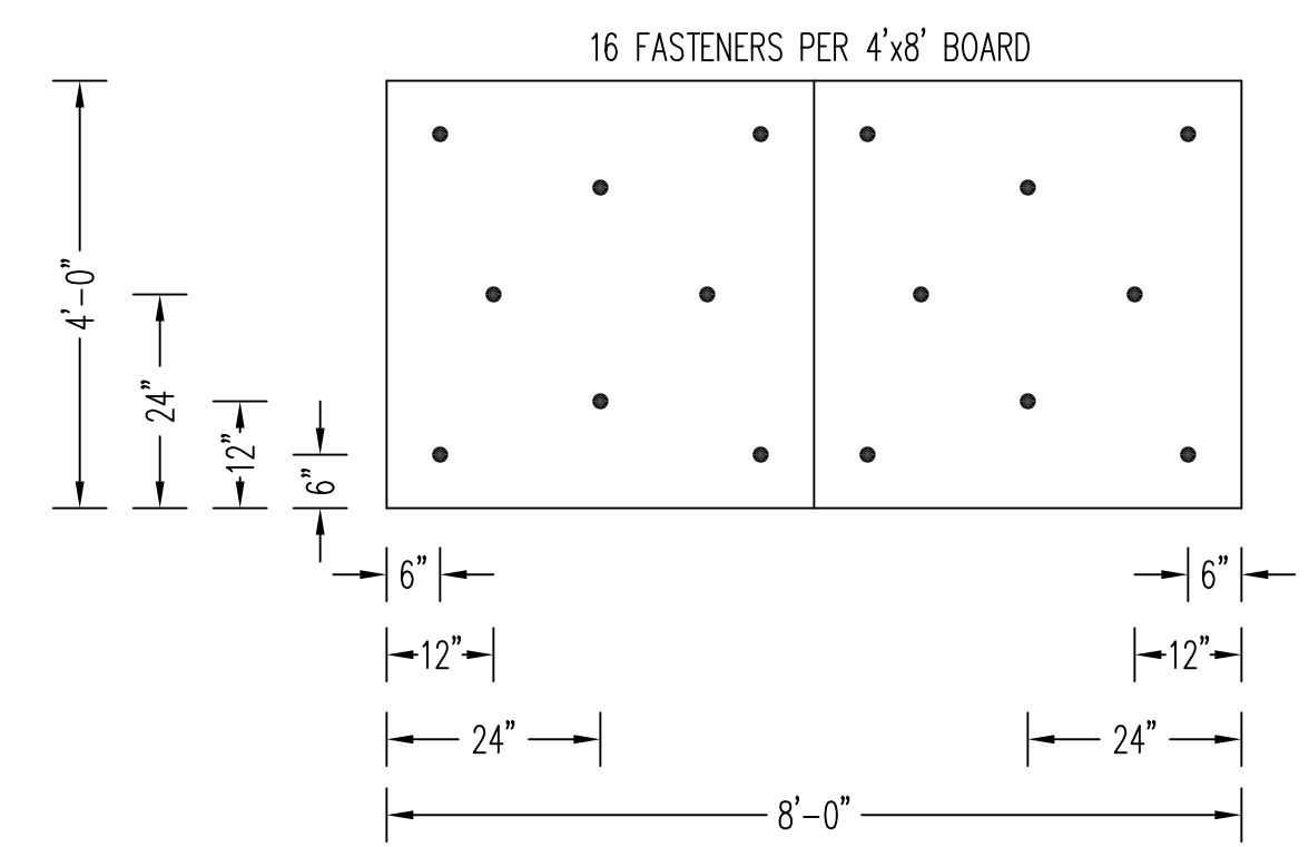
3 FIELD INSULATION FASTENER LAYOUT G1 | D4 NO SCALE
