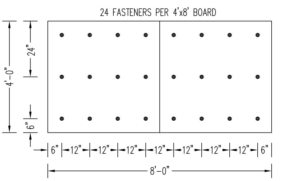
4 CORNER & PERIMETER INSULATION FASTENER LAYOUT G1 | D4 NO SCALE
