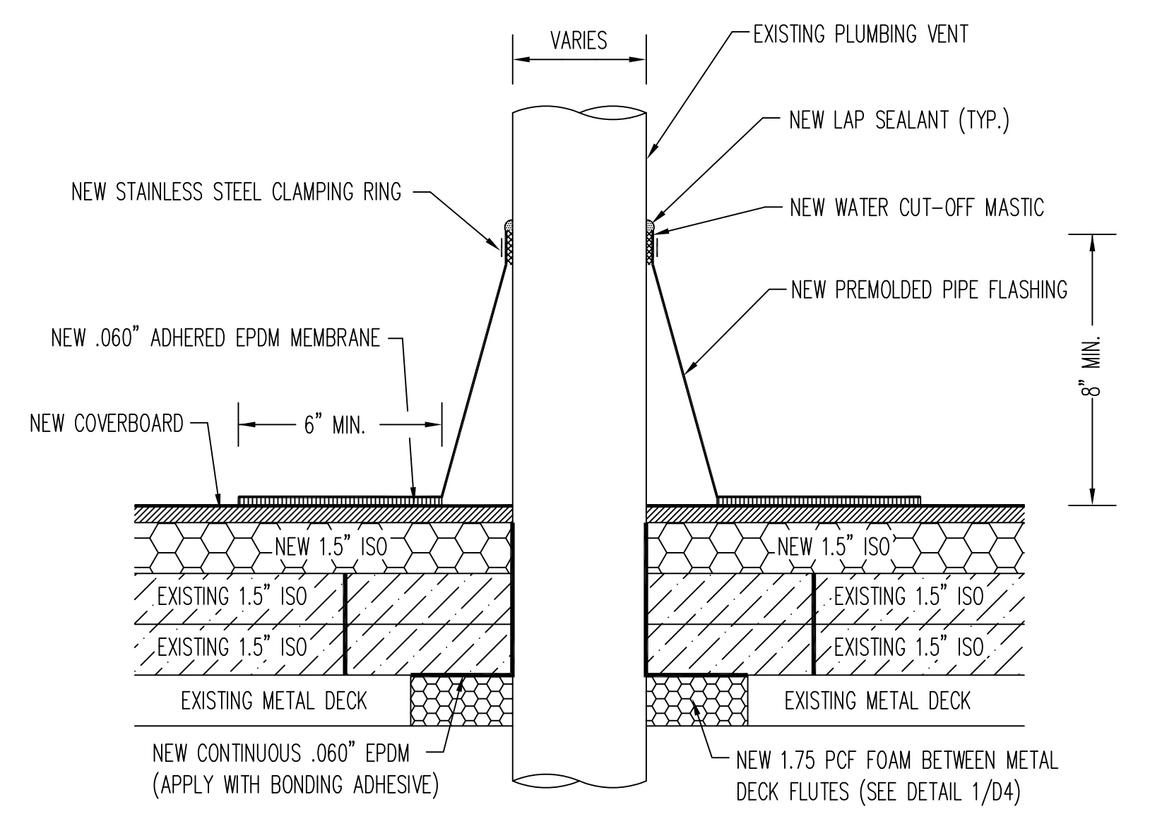
3 PLUMBING VENT DETAIL SCALE: 3" = 1'-0"
