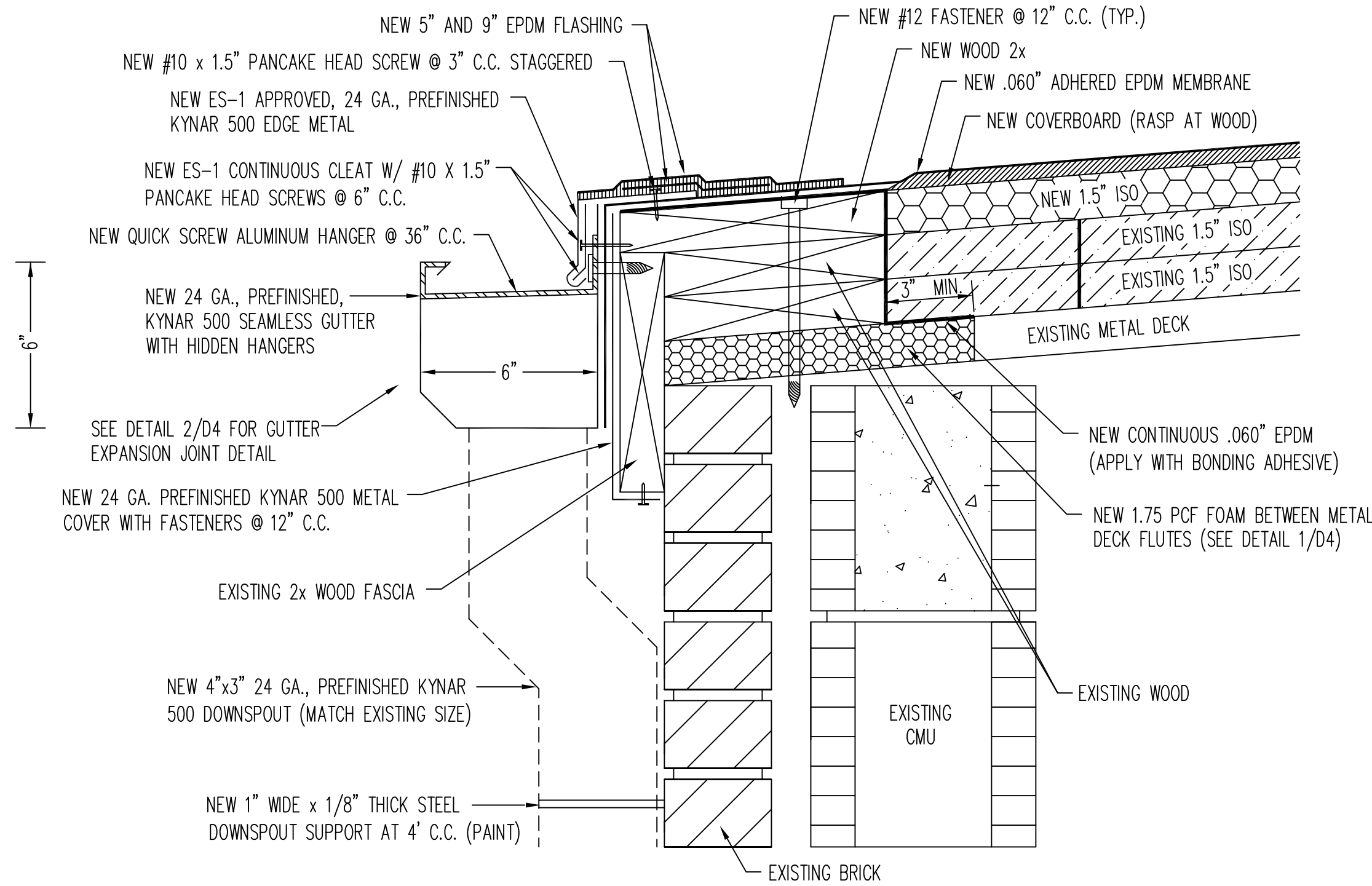
1 GUTTER DETAIL (METAL DECK) (GDS) SCALE: 3" = 1'-0"
