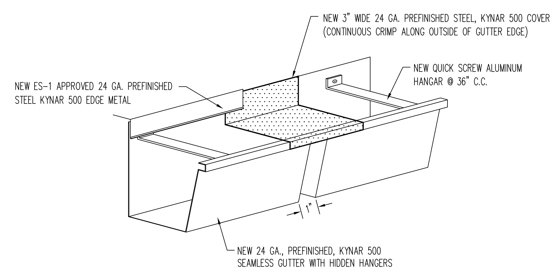
2 GUTTER EXPANSION DETAIL G1 | D4 SCALE: 3" = 1'-0"
