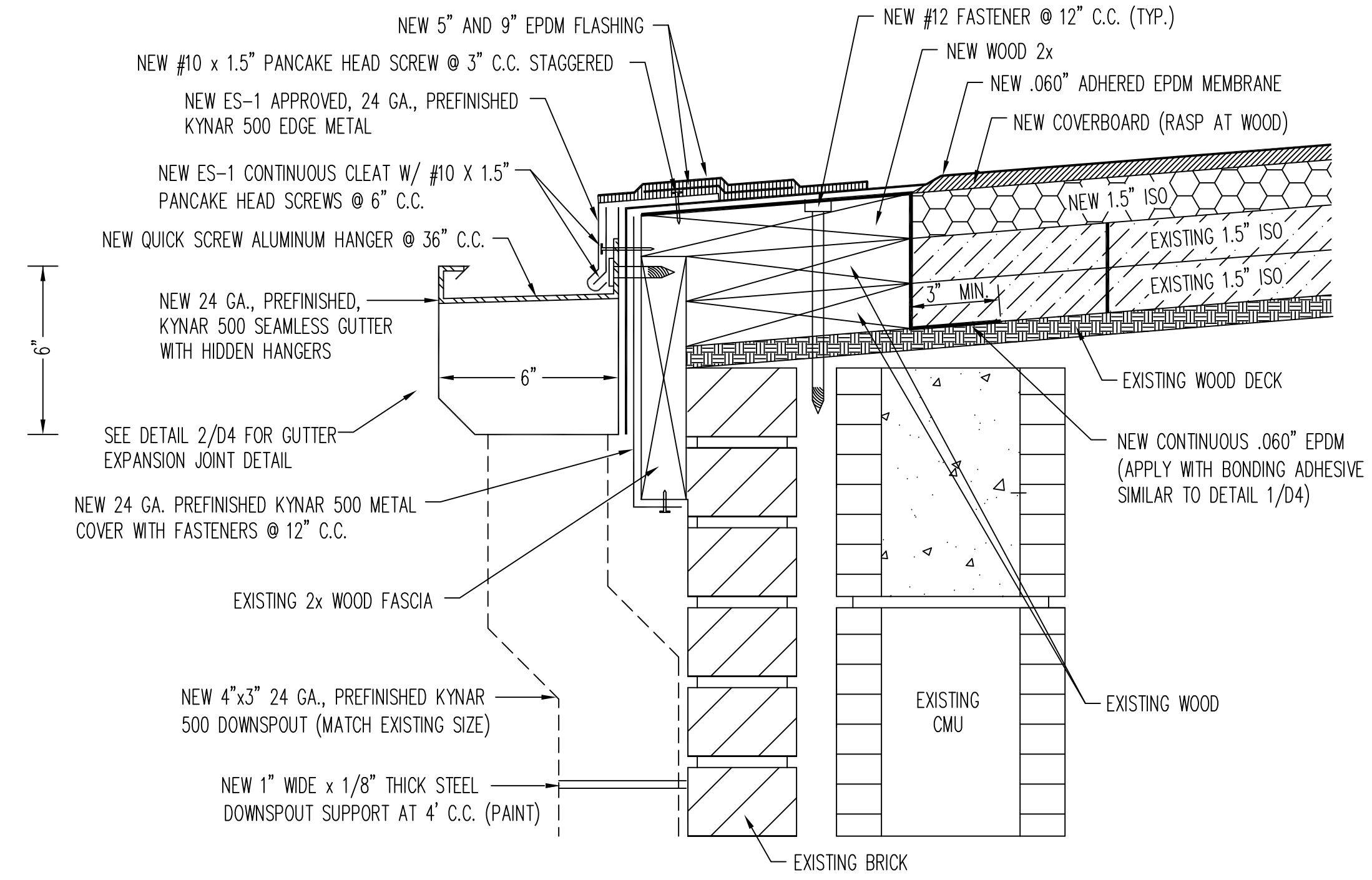
2 GUTTER DETAIL (WOOD DECK) (GDS) SCALE: 3" = 1'-0"
