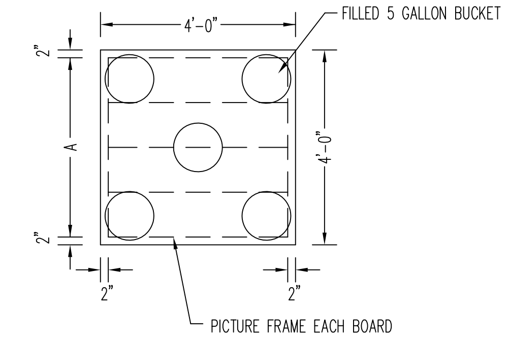
5 TYPICAL INSULATION ADHESIVE PATTERN G1 | D4 NO SCALE
